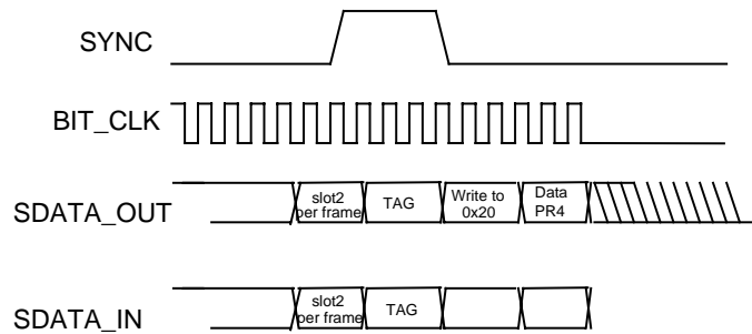
Figure 10. STAC9708/11 Powerdown Timing
