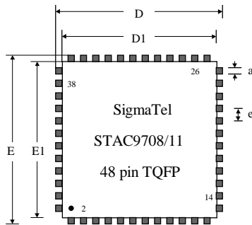
Figure 1. Package Outline
